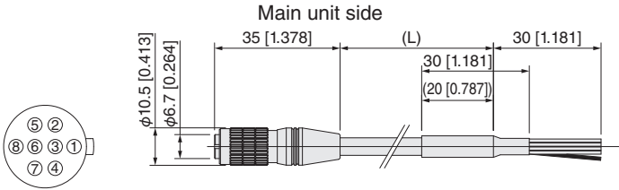
Pin location
