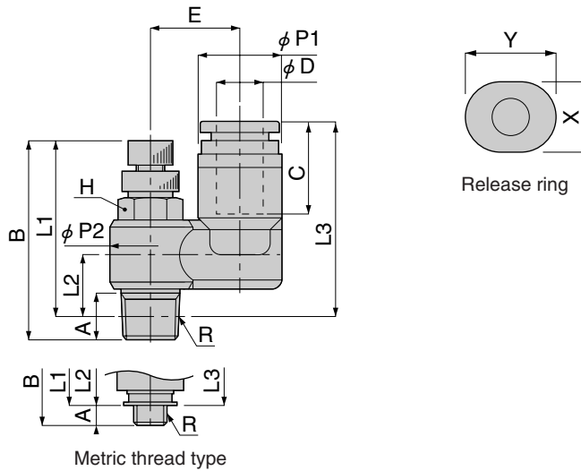
Metric thread type
