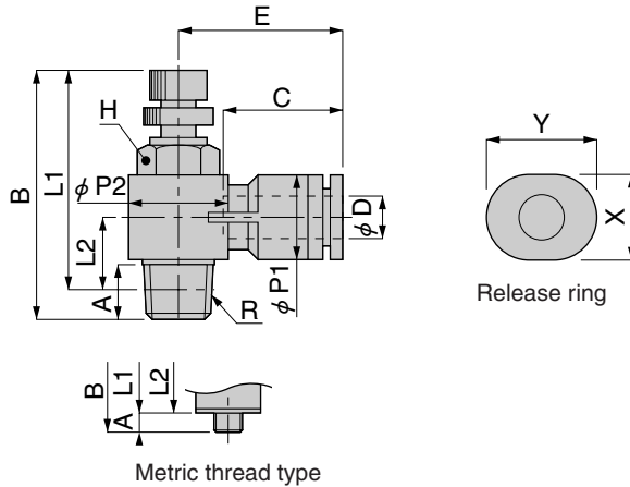
Metric thread type
